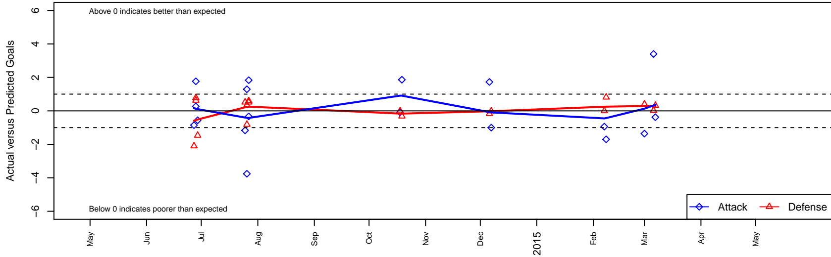
Surrey United 2001B Dots are actual minus expected GF (blue circles) and GA (red triangles). Blue line is smoothed change in attack strength. Red is smoothed change in defense strength.
